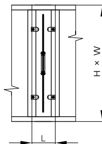
FROST PROTECTION GRID (FPG)
