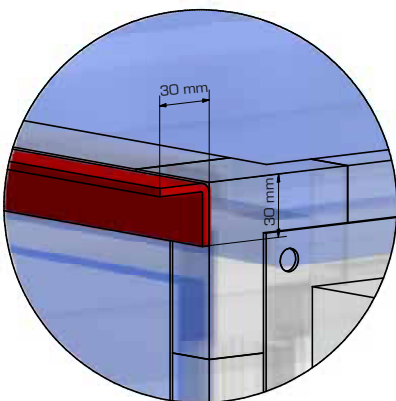
Ceiling mounting brackets
