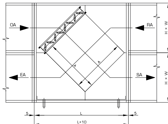
CROSS FLOW PLATE HEAT EXCHANGER (PHE)
