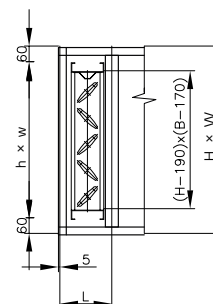
EXTERNAL DAMPER (ED)
