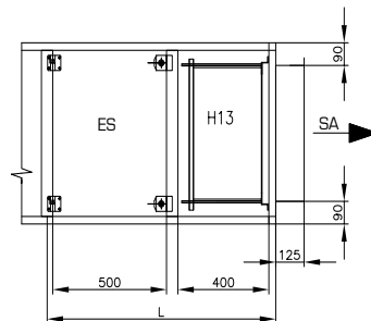
HIGH EFFICIENCY FILTER (HEF)
