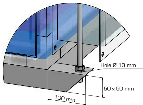
Console ceiling mounting
