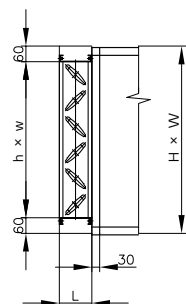
INTERNAL DAMPER (ID)
