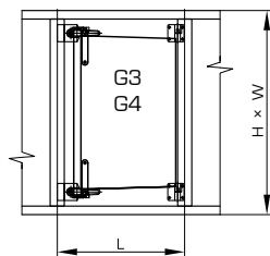
COARSE DUST FILTER (CF)
